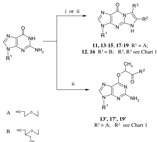
Scheme 1. Reagents: (i) (1) NaH, DMF, R 2 COCH 2 Br, (2) NH 4 OH; (ii) (1) NaH, DMF, R 2 COCH(Br)CH 3 , (2) NH 4 OH.
